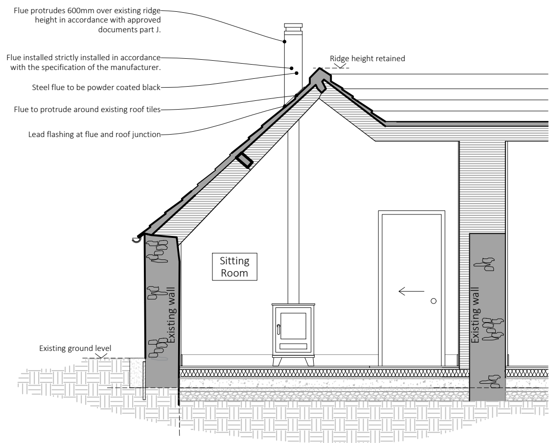
Proposed Section C-C - 1:50
