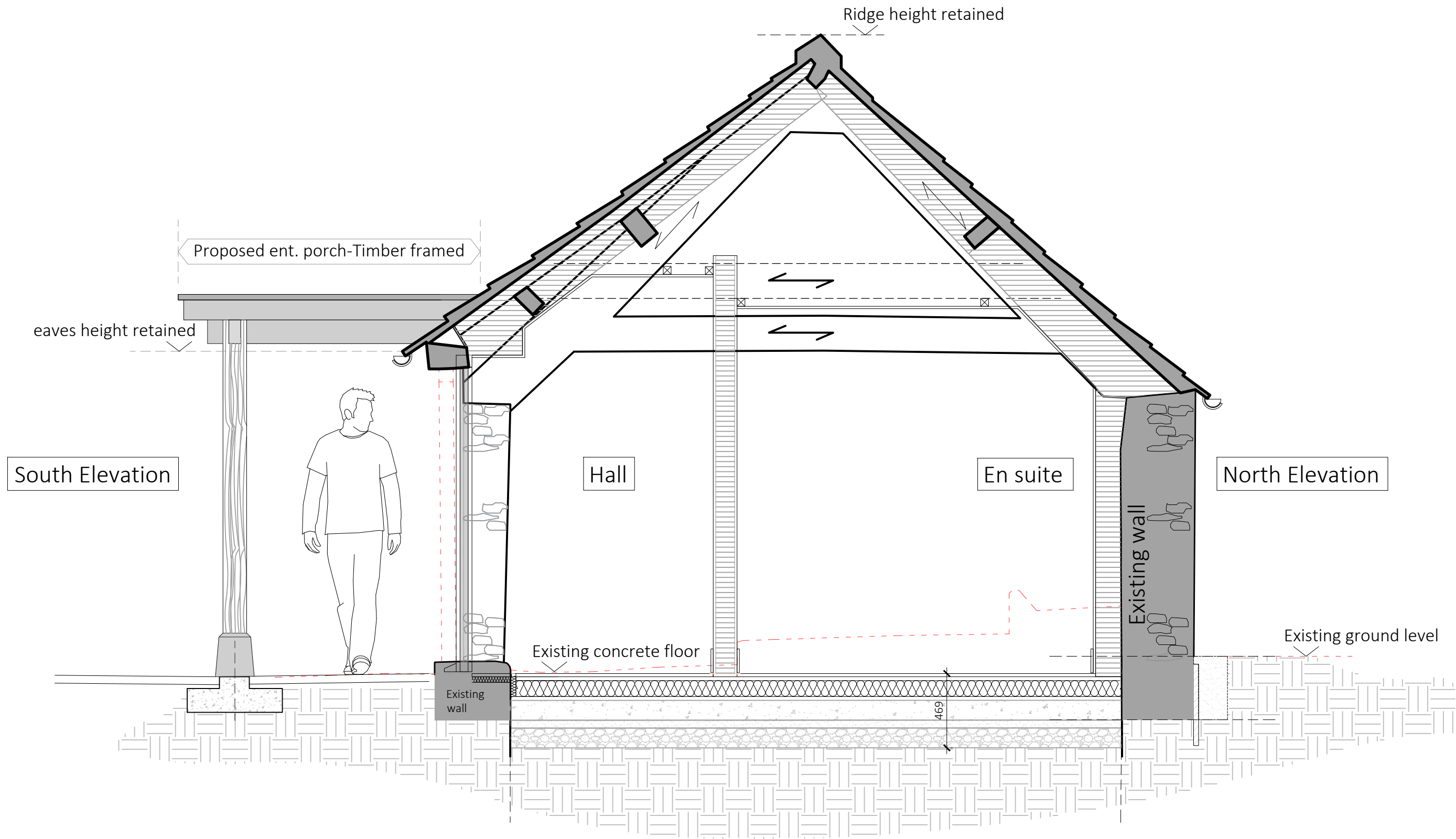
Section BB
