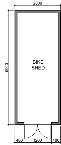
FLOOR PLAN SCALE 1:100 @A4
