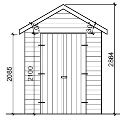
FRONT ELEVATION SCALE 1:100 @A4
