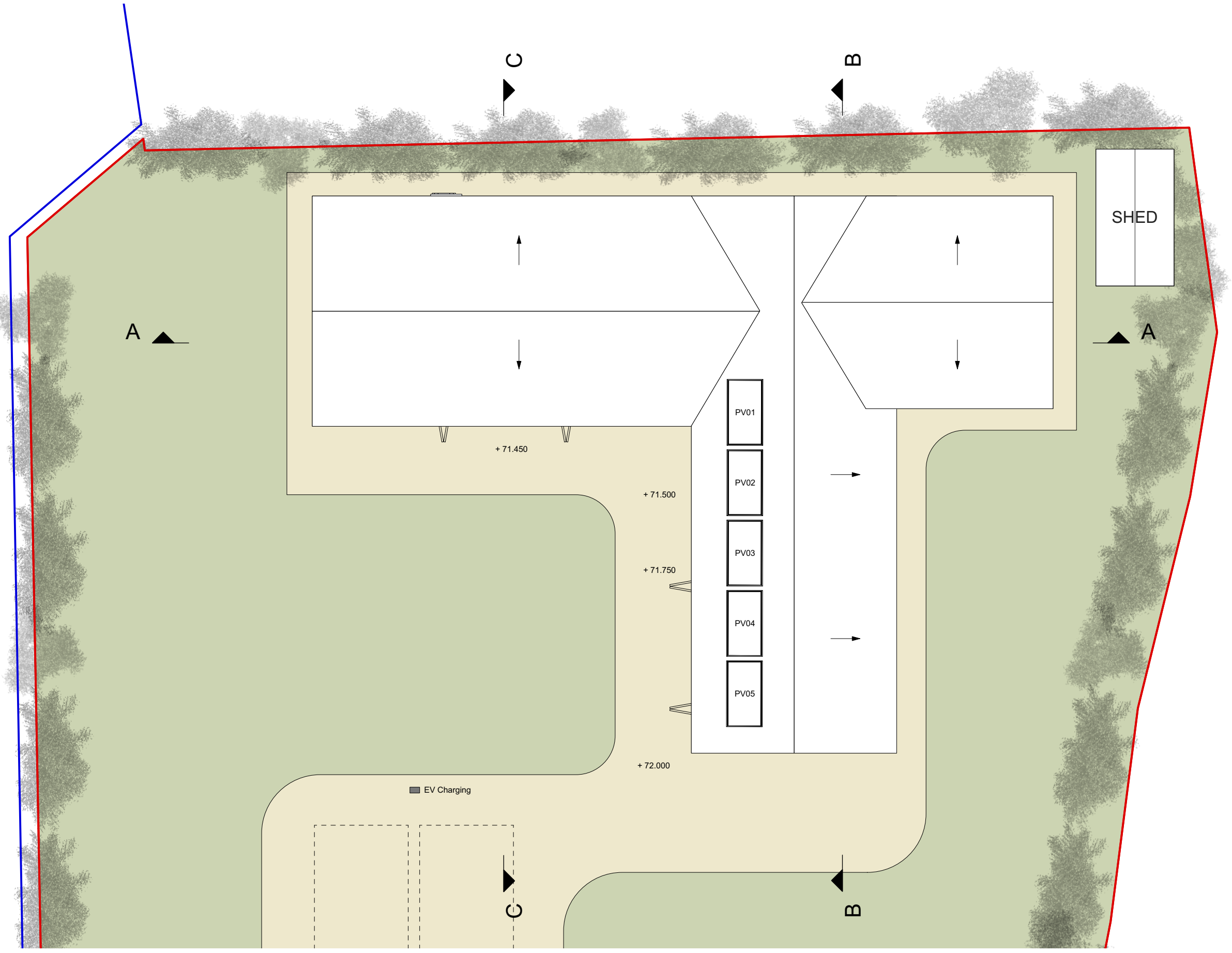
PROPOSED ROOF PLAN 1:100 @ A3
