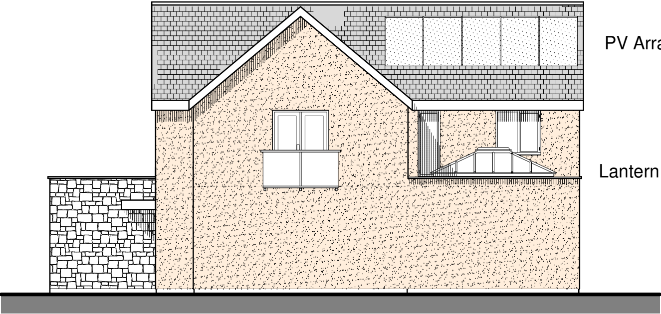
SOUTH ELEVATION
