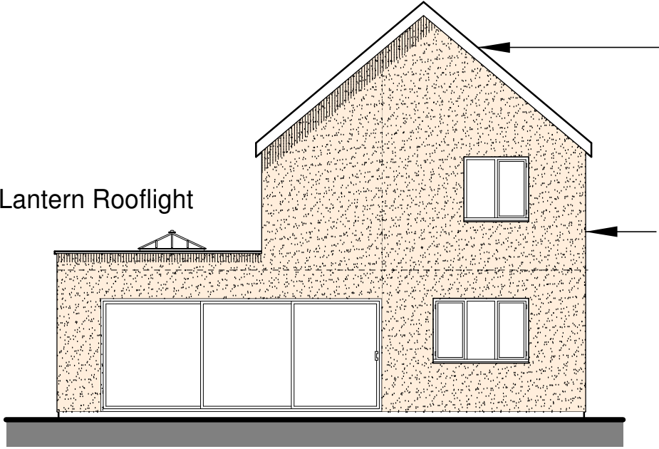
EAST ELEVATION
