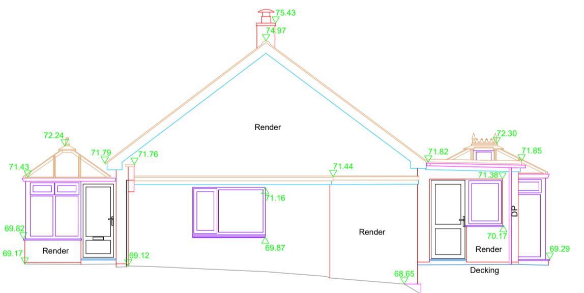
South Elevation
