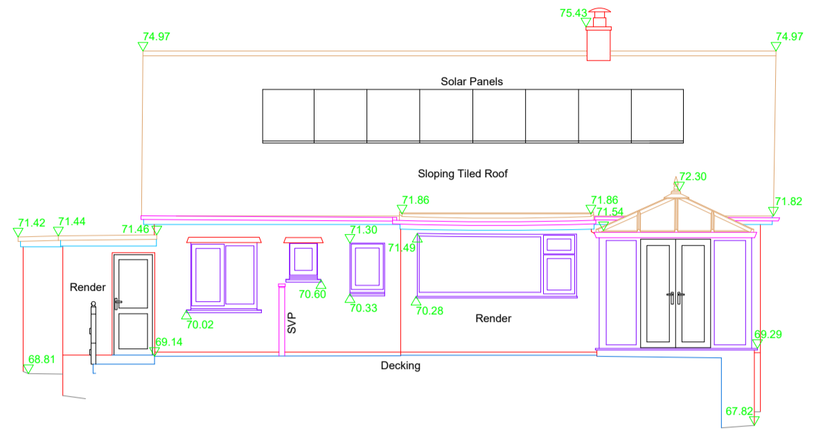
East Elevation
