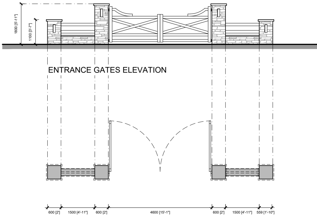
ENTRANCE GATES PLAN
