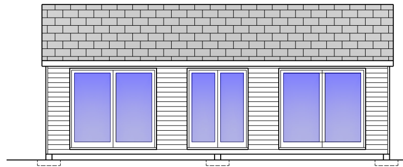
E2 Front Elevation Proposed 1:100
