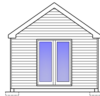
E3 Side Elevation Proposed 1:100
