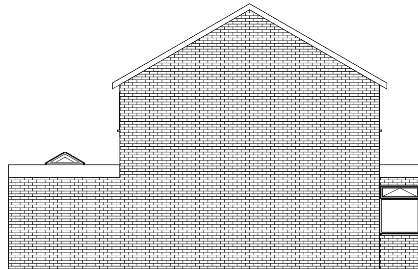
4 Proposed Side B Elevation 1 : 100
