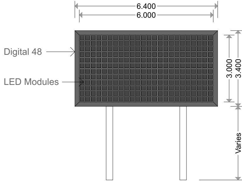
FRONT ELEVATION
