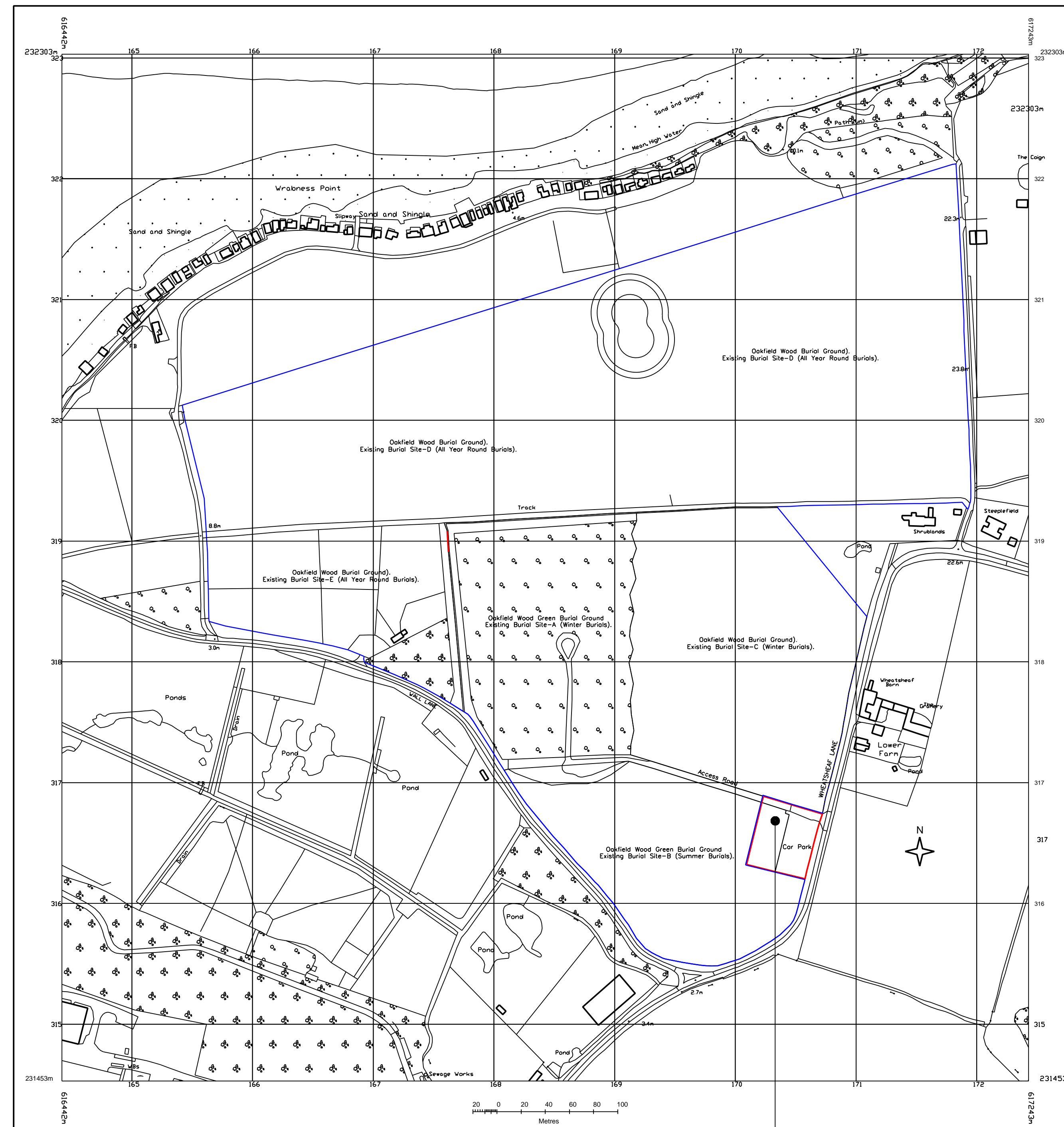
SITE LOCATION PLAN SCALE 1:2500
