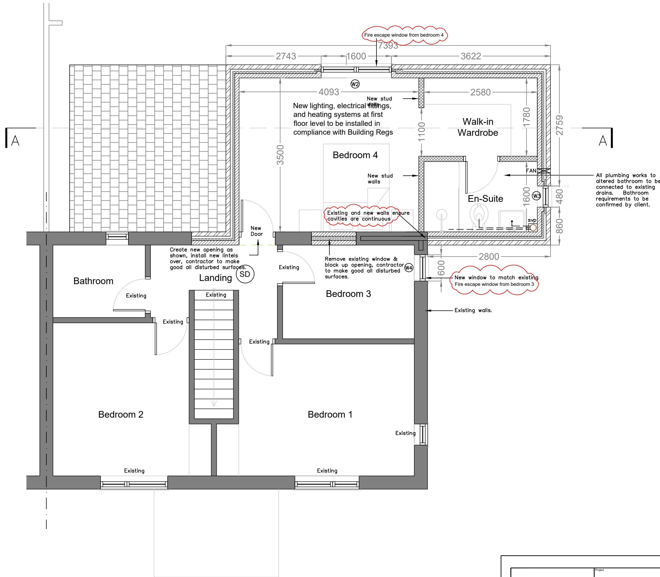
Proposed First Floor Plan 1:50 @ A3
