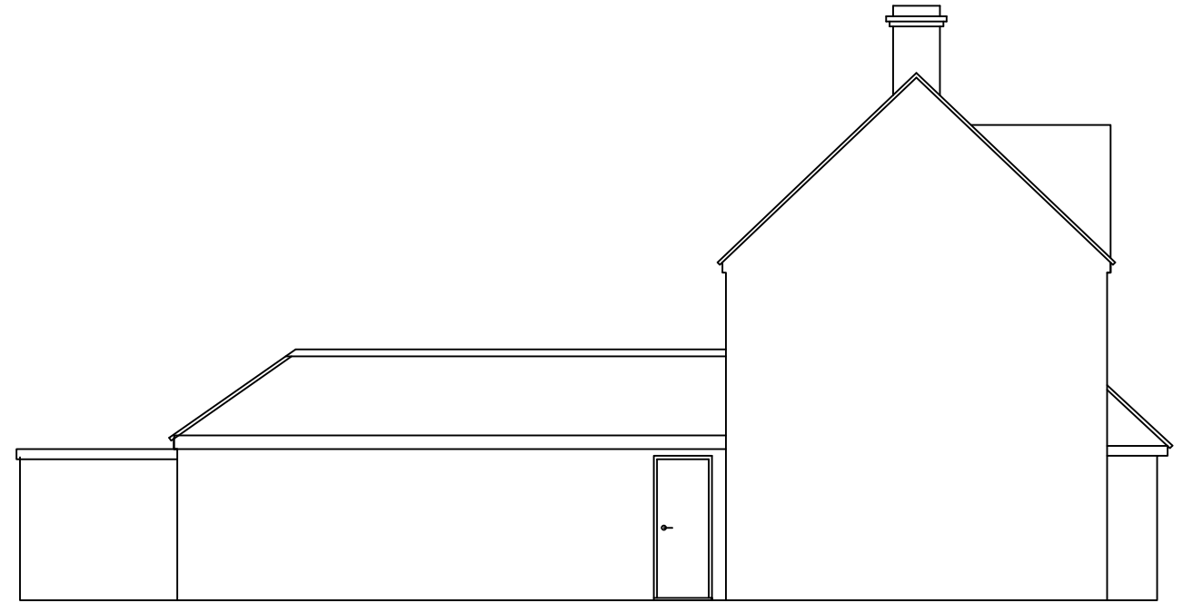
Proposed Side (eastern) Elevation
