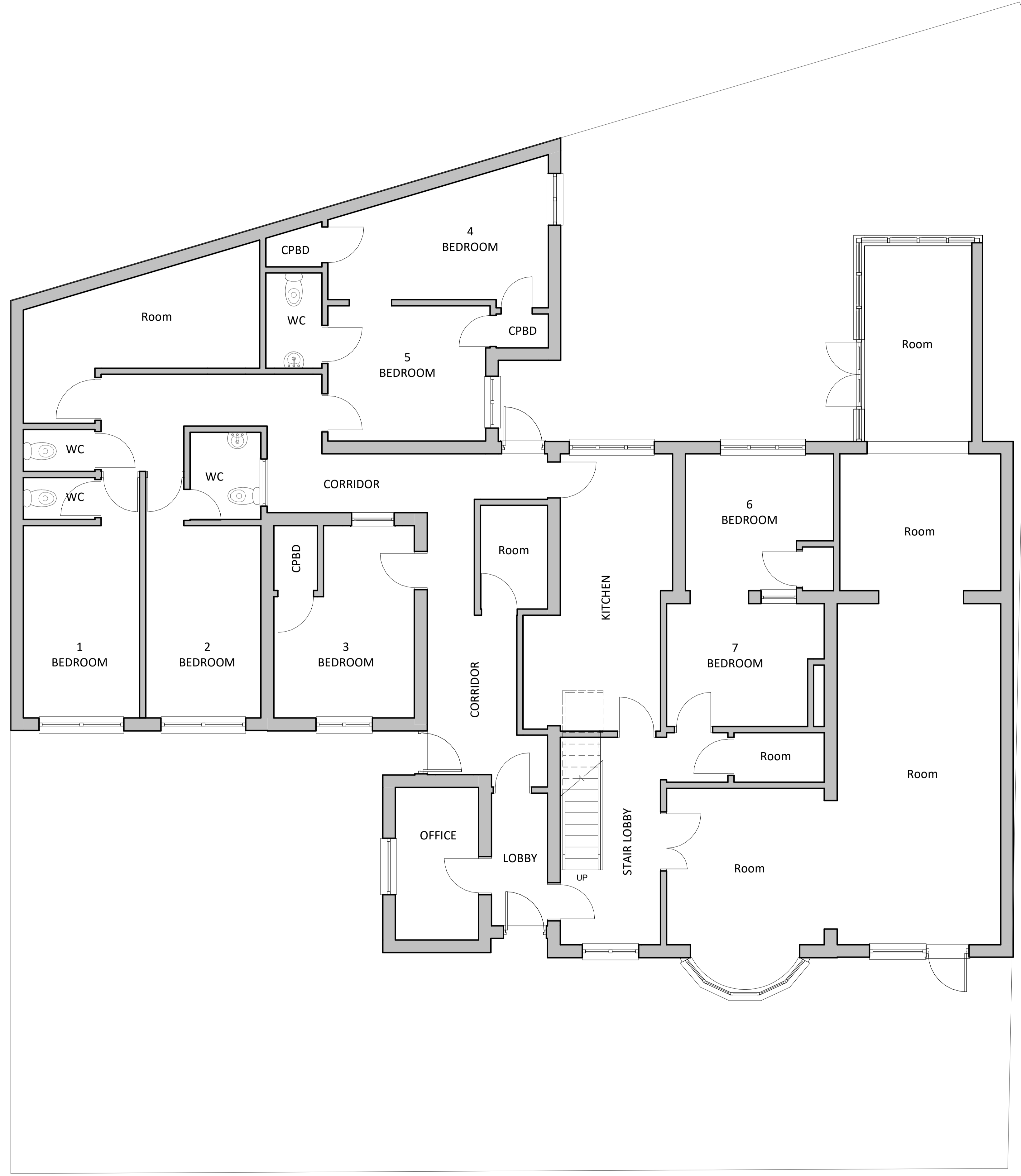
1 EXISTING - GROUND FLOOR PLAN 1 : 50
