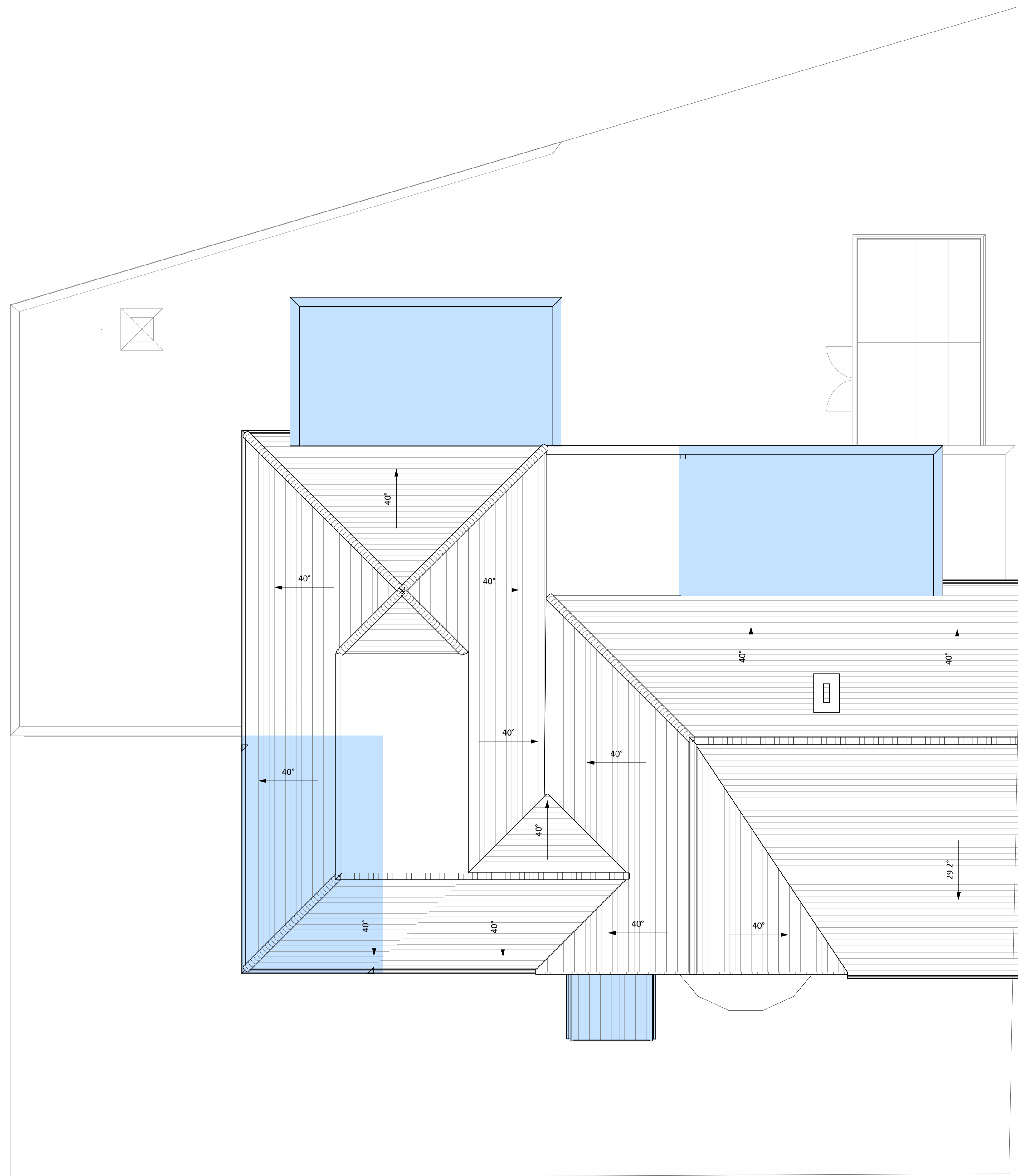
1 | PROPOSED - ROOF PLAN - COMPLETE 1 : 50
