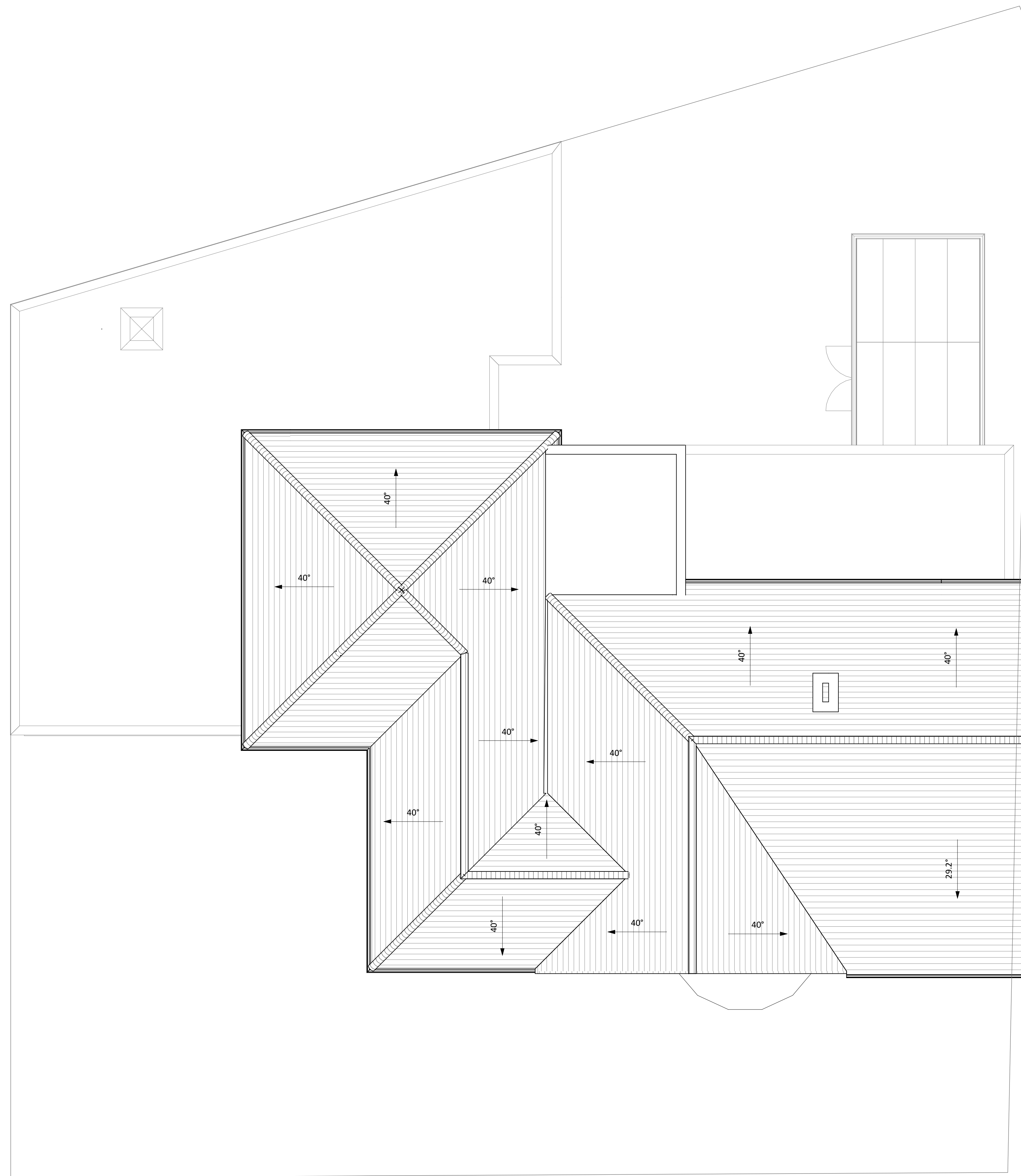
1 EXISTING - ROOF - PLAN 1 : 50
