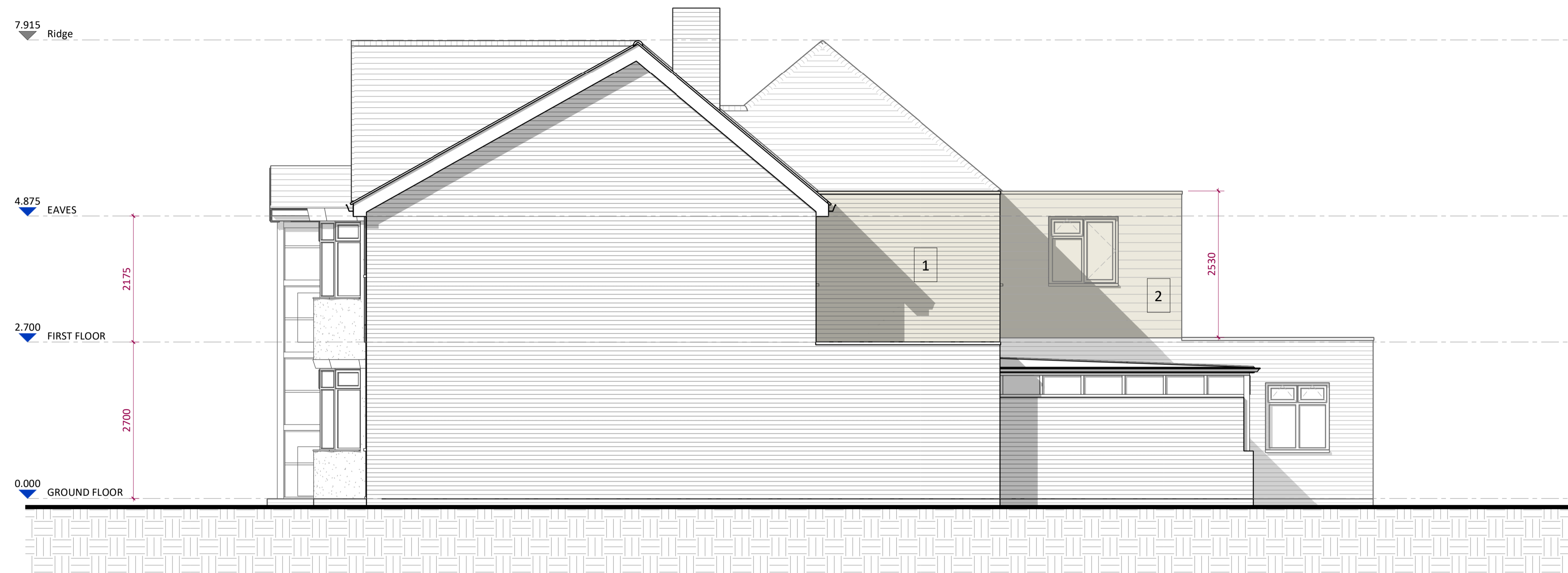
1 SOUTH - ELEVATION - COMPLETE 1 : 50
