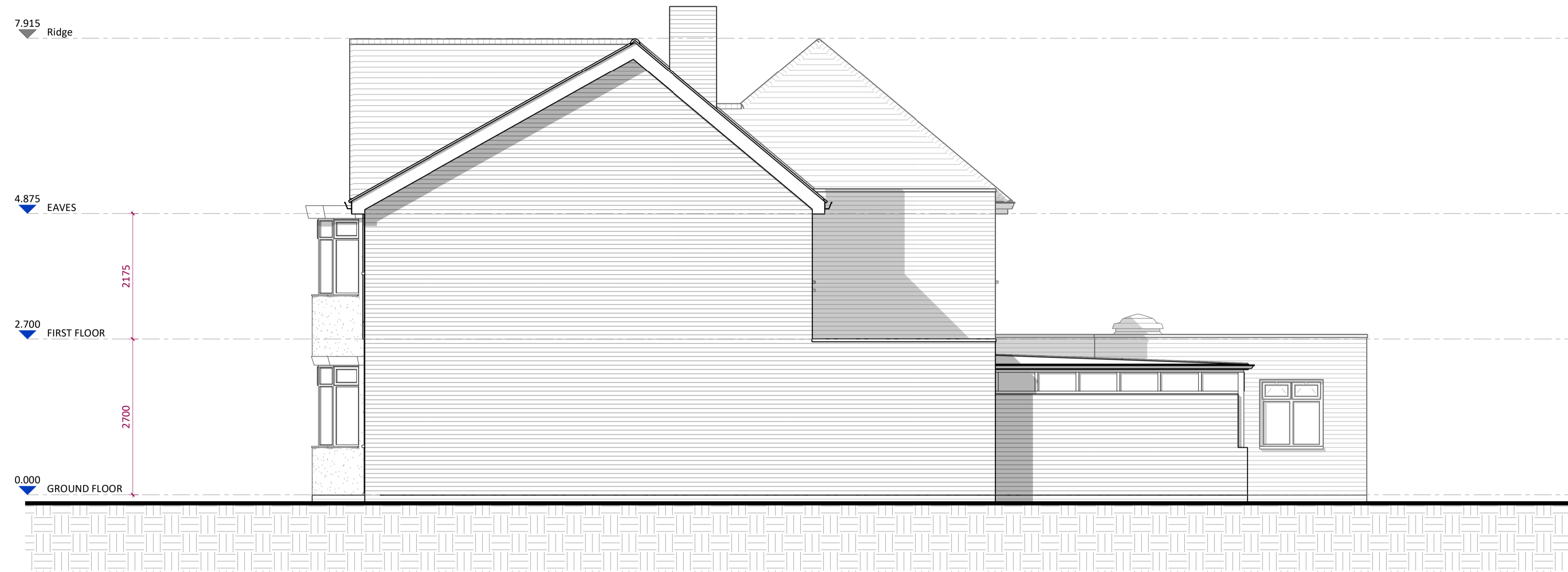
1 SOUTH - ELEVATION 1 : 50
