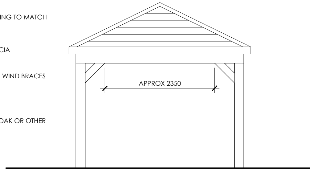
FRONT AND REAR ELEVATIONS
