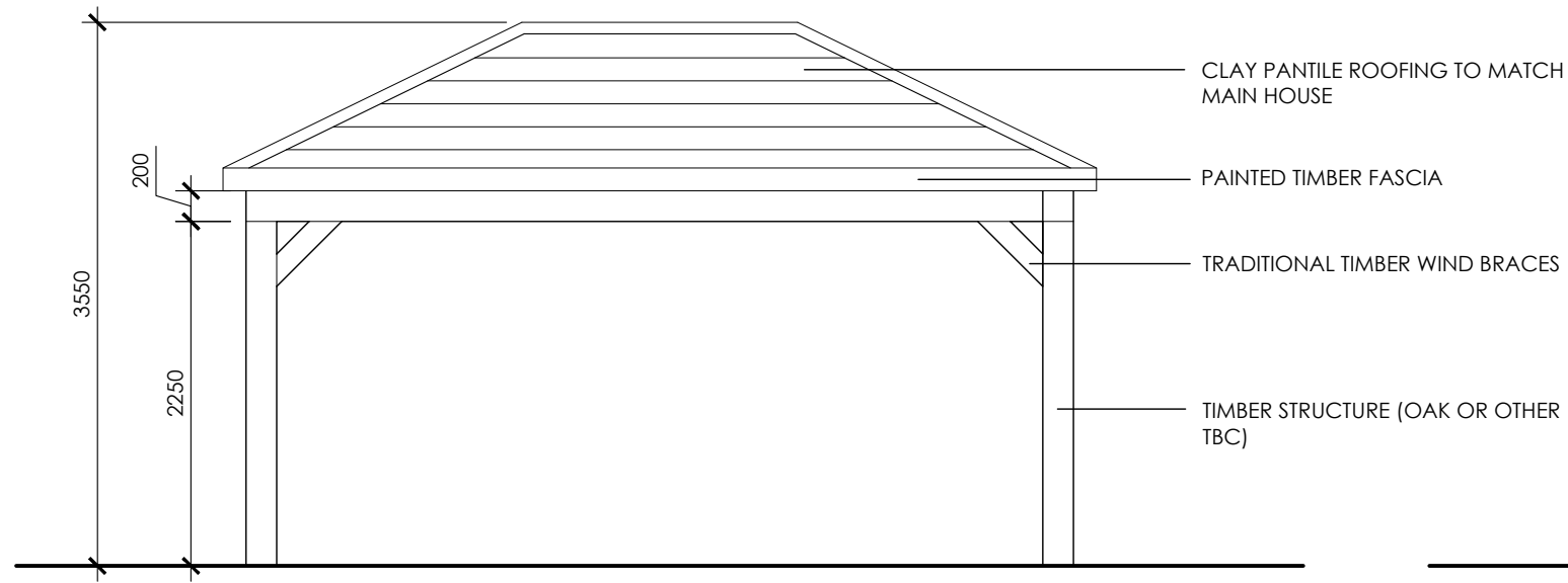
SIDE ELEVATIONS
