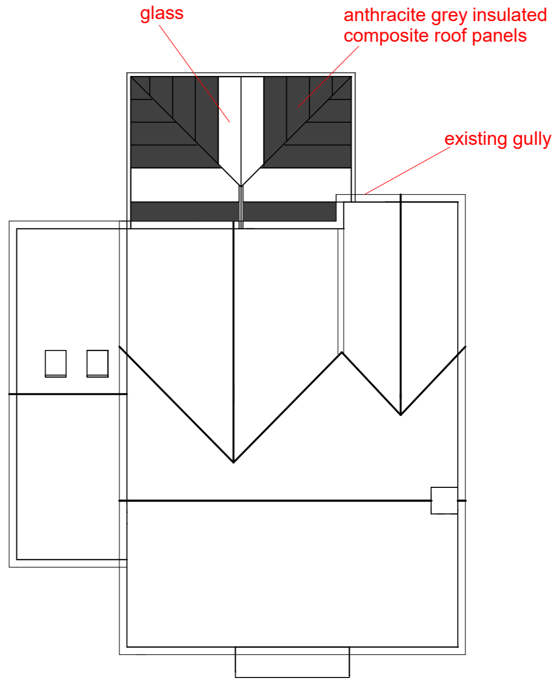
ROOF PLAN
