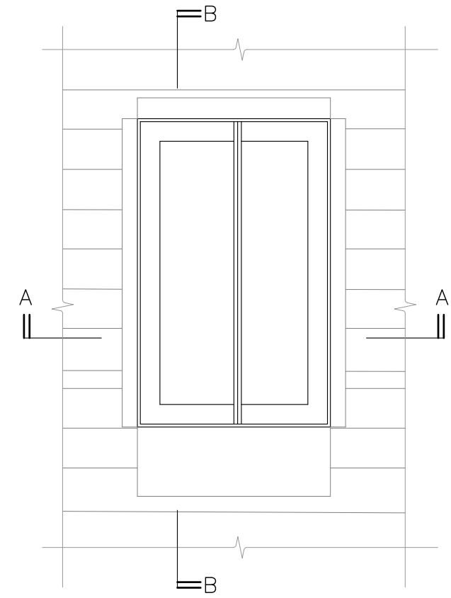
Proposed Conservation Rooflight Detail Typical Elevation (not to scale)
