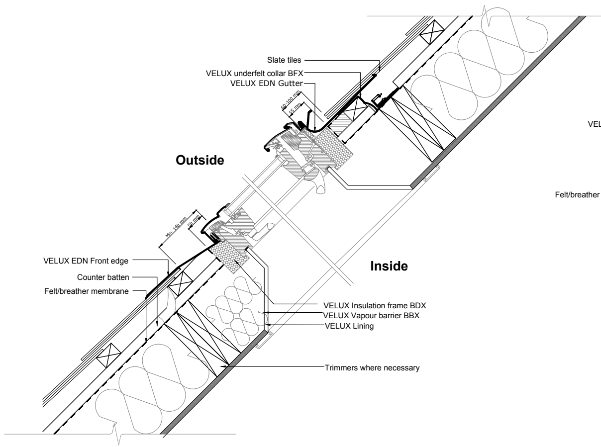
Proposed Conservation Rooflight Detail Section BB
