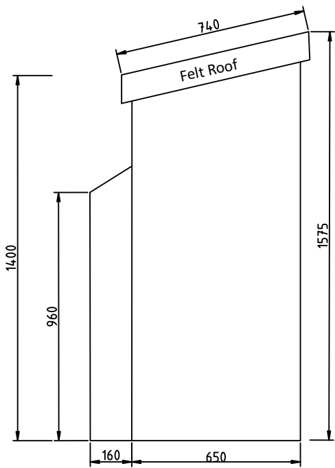
Left Elevation
