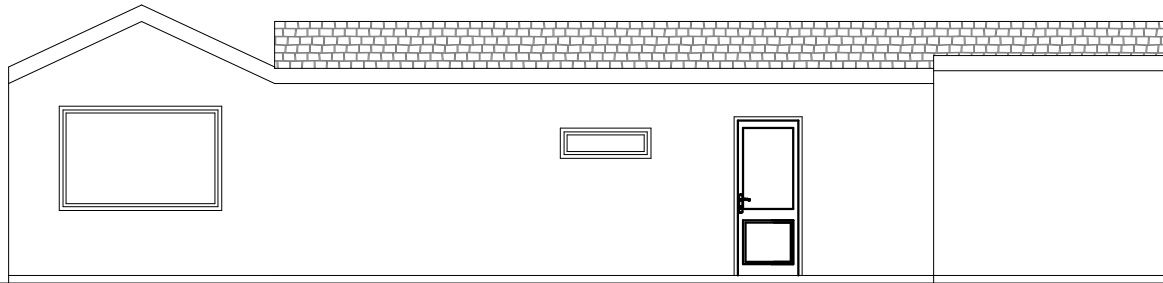
SOUTH SIDE ELEVATION
