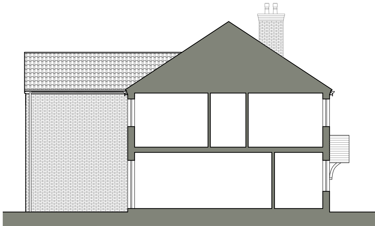
03 PROPOSED SECTION THRU HOUSE 1:100
