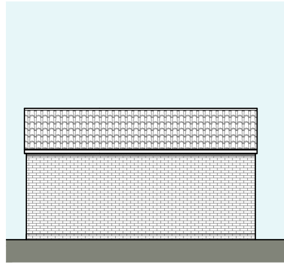
02 PROPOSED GARAGE ELEVATIONS 1:100
