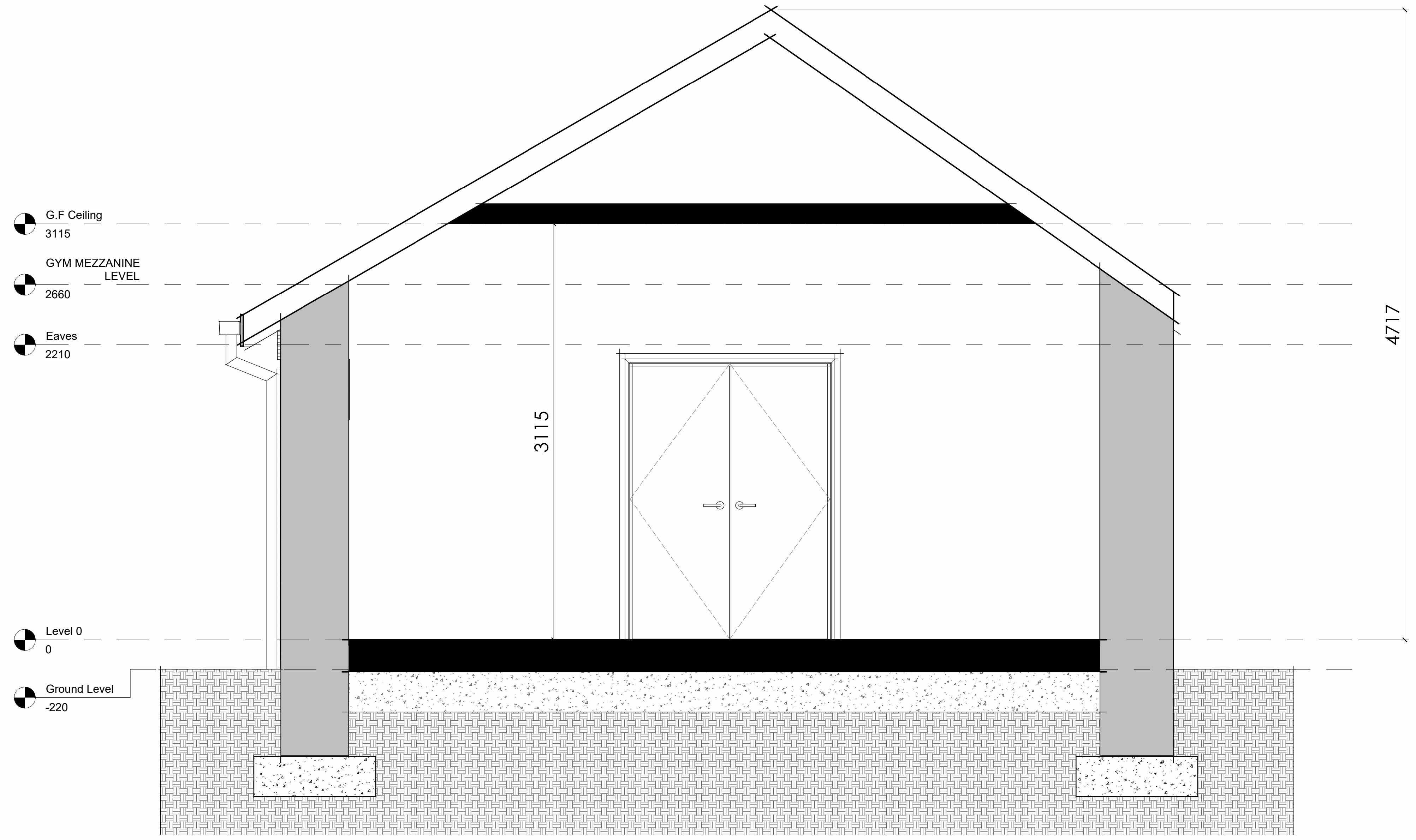
1 EXISTING SECTION THROUGH GYM 1 : 20
