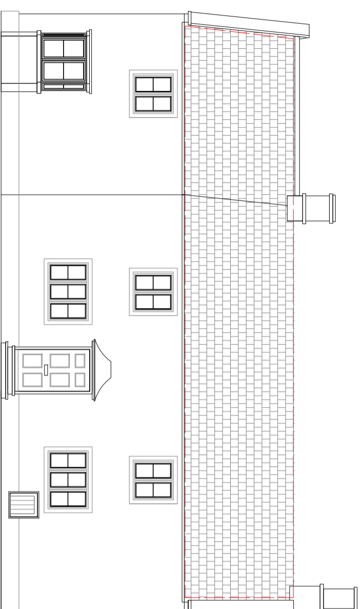
Front Elevation
