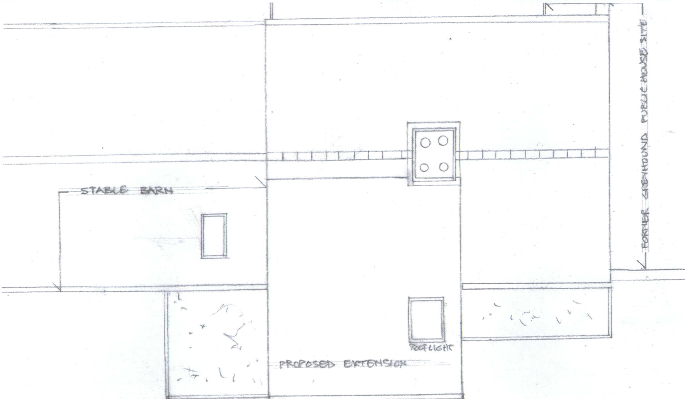
ROOF PLAN AS PROPOSED 29 THE STREET WEST RAINHAM SCALE 1:50 DRWG No 216
