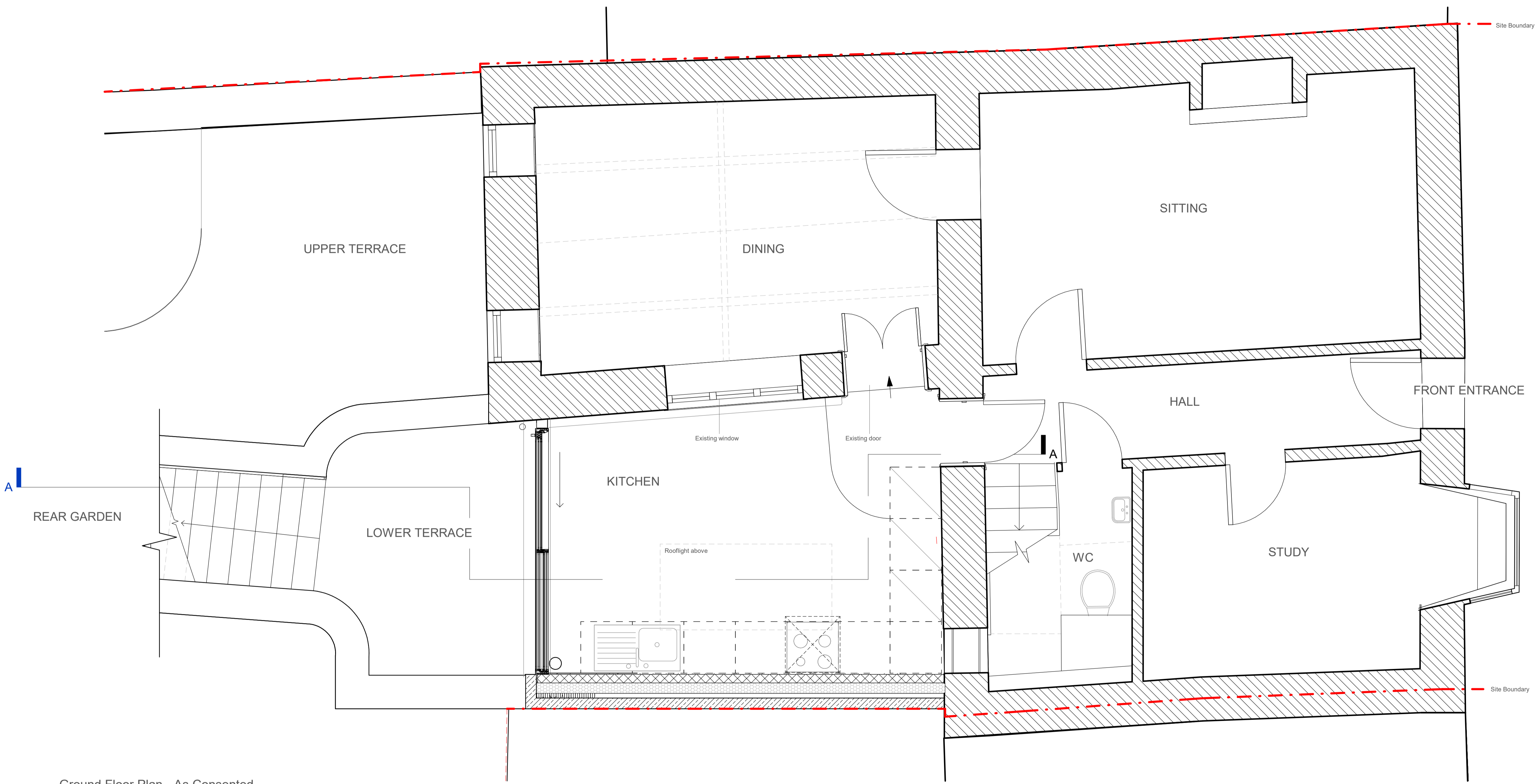
Ground Floor Plan - As Consented
