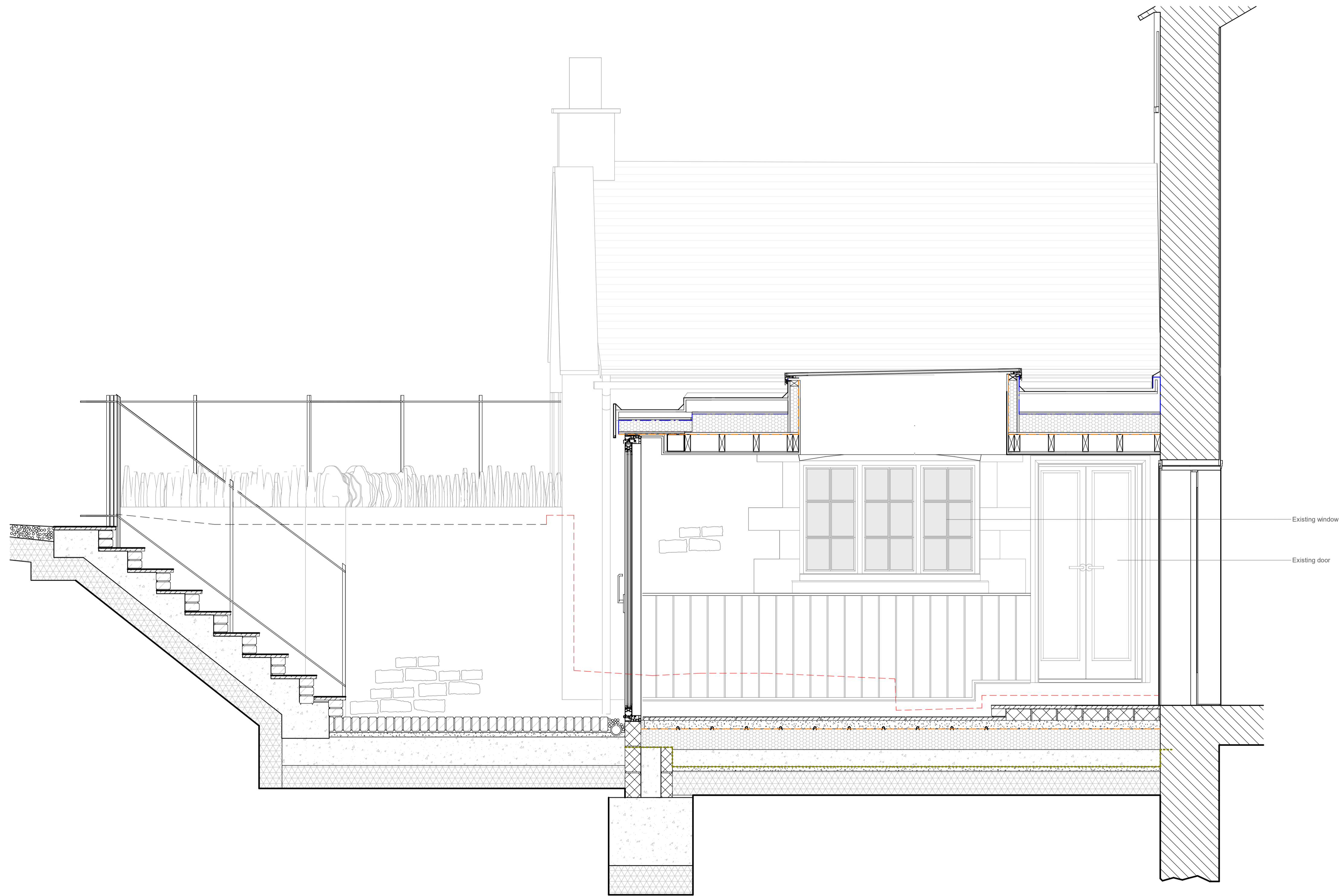
Section AA - As Consented 1:20
