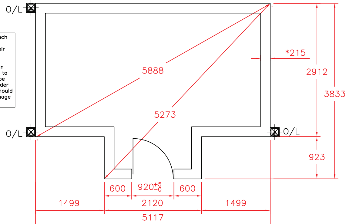
GROUND PLAN.
