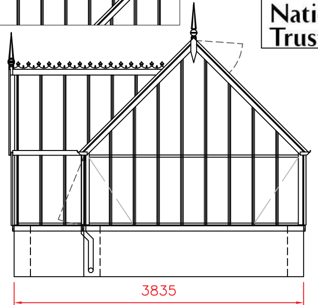
GABLE ELEVATION
