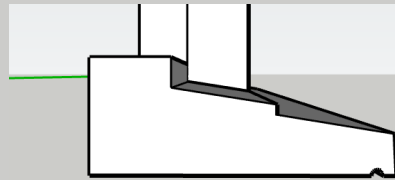
Frame Cill with 9 Degree bevel and capillary groove
