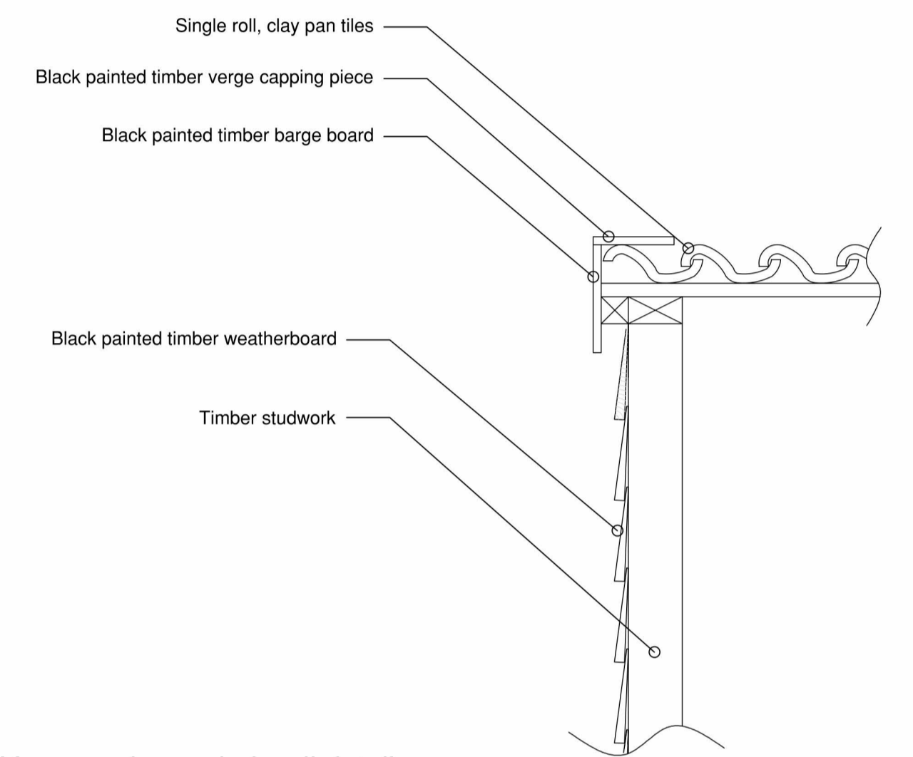
Verge and spandrel wall detail Scale 1:10
