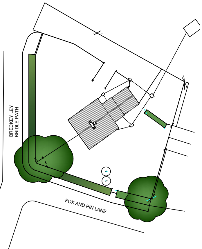
09 SITE PLAN 1:500 001 COURT FARM COTTAGE
