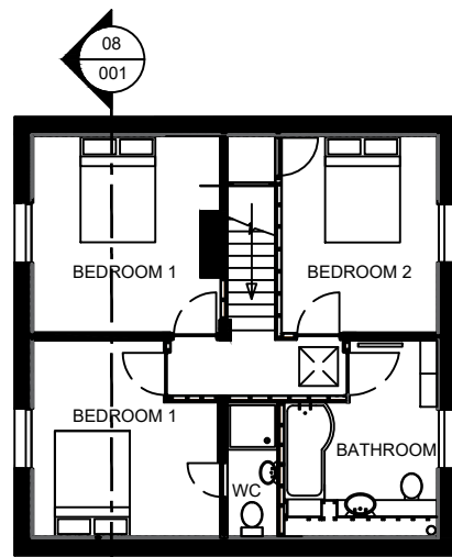
05 FIRST FLOOR PLAN 1:150 001 COURT FARM COTTAGE
