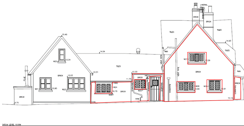
SOUTH-EAST ELEVATION (SIDE FACING GARDEN)
