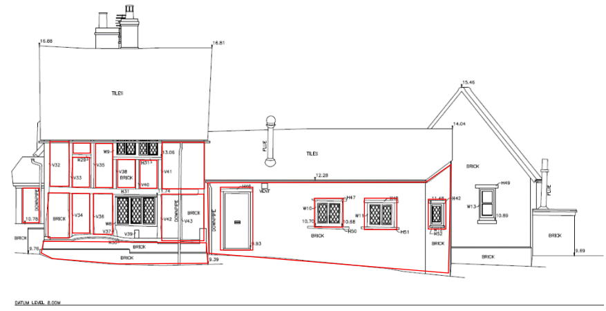
NORTH-WEST ELEVATION (SIDE FACING ROAD)
