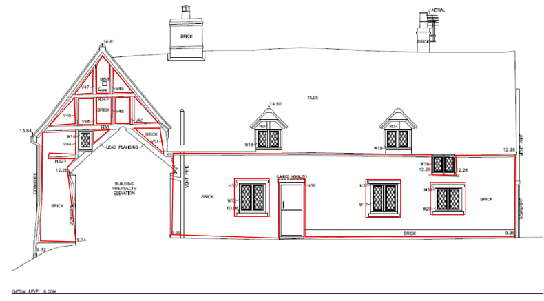
SOUTH-WEST ELEVATION (INNER COURTYARD)
