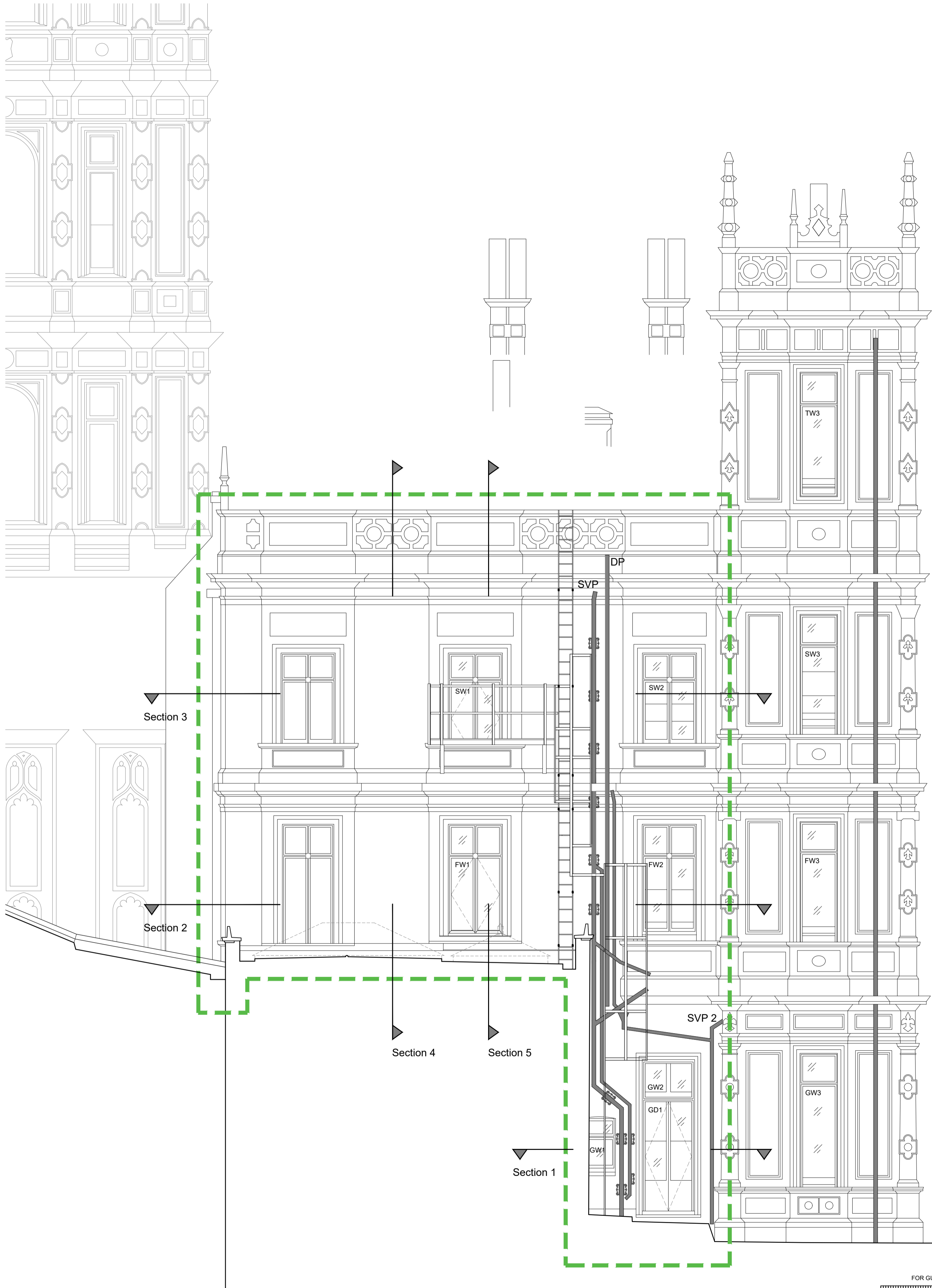
Key Elevation (West) Scale 1:50
