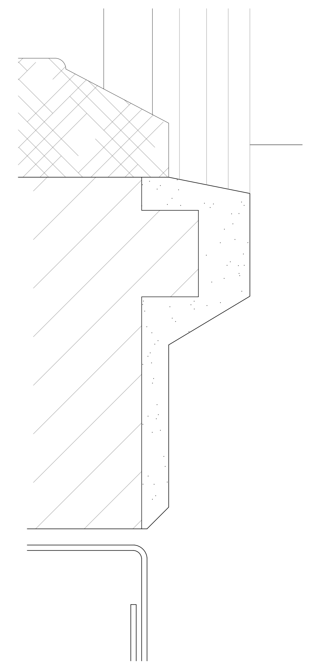
Detail N as Existing Scale 1:2
