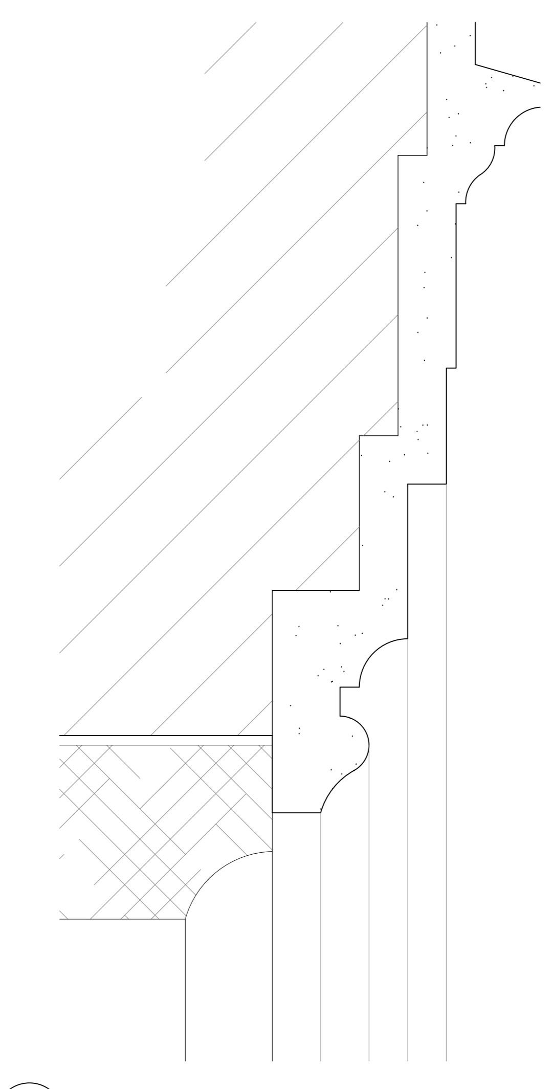
Detail M as Existing Scale 1:2
