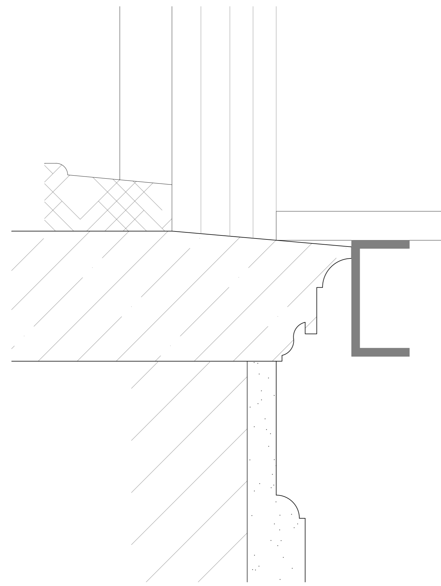
Detail K as Existing Scale 1:2
