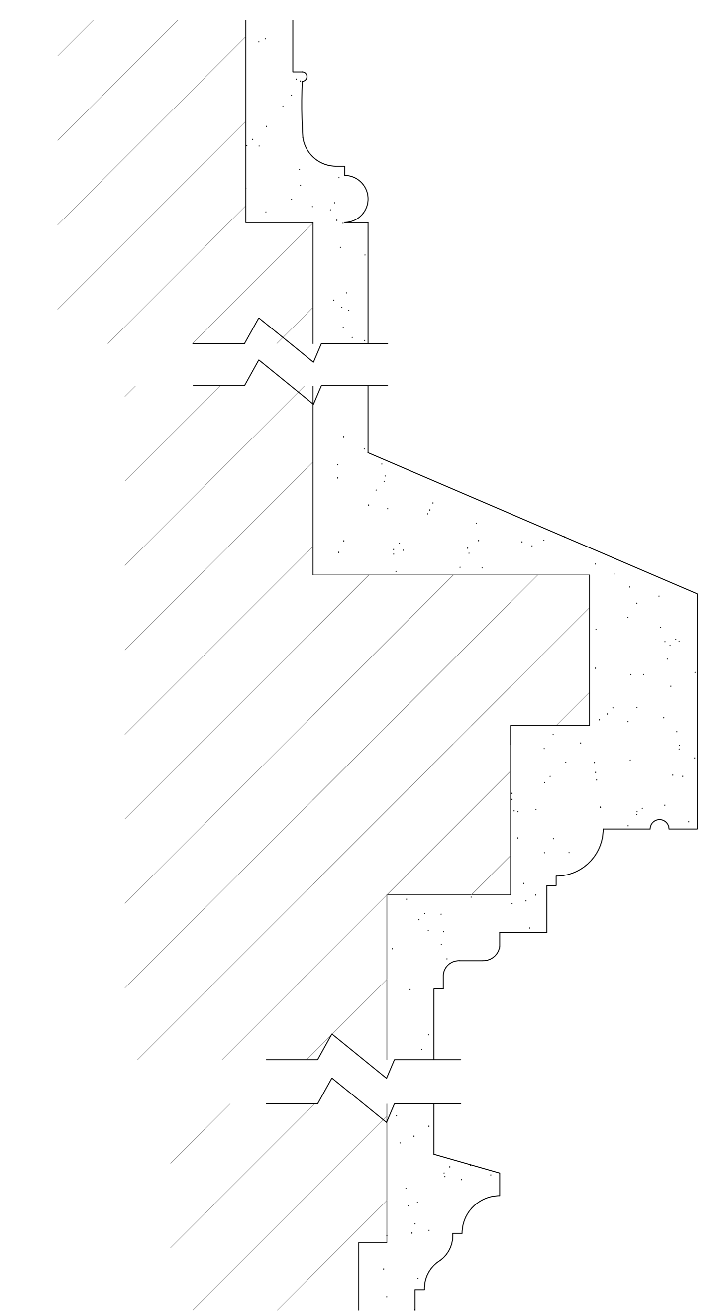
Detail H as Existing Scale 1:2
