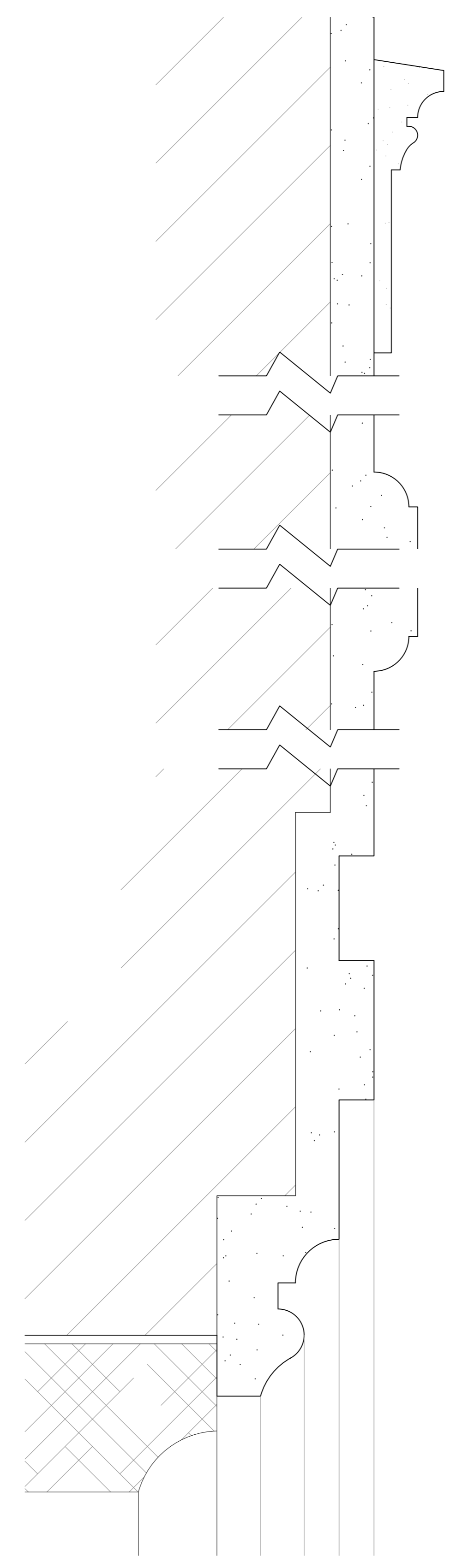
Detail J as Existing Scale 1:2
