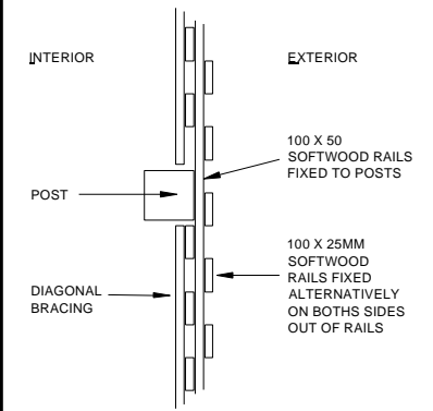
PLAN DETAILS SCALE - 1:25
