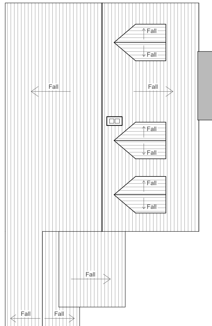
Roof Plan
