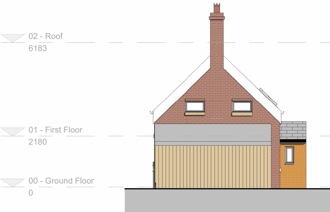
Left Side Elevation - Proposed
