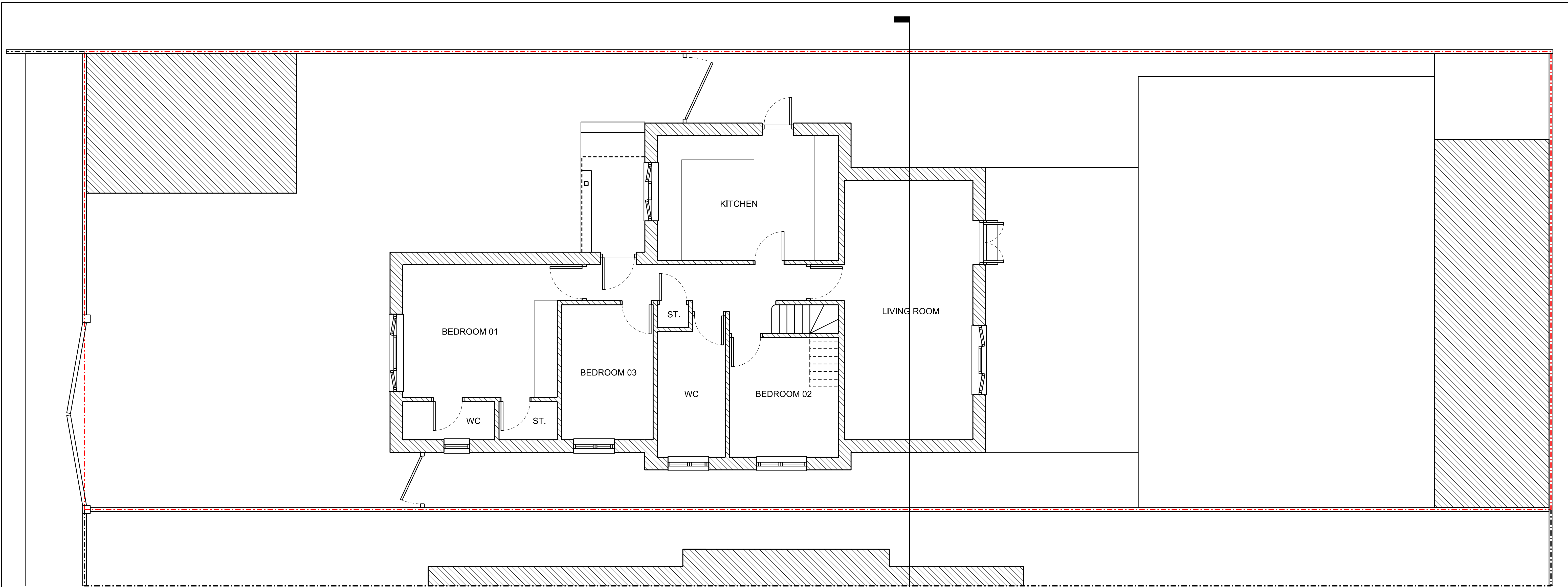
PROPOSED GROUND FLOOR PLAN 1.50@A1
