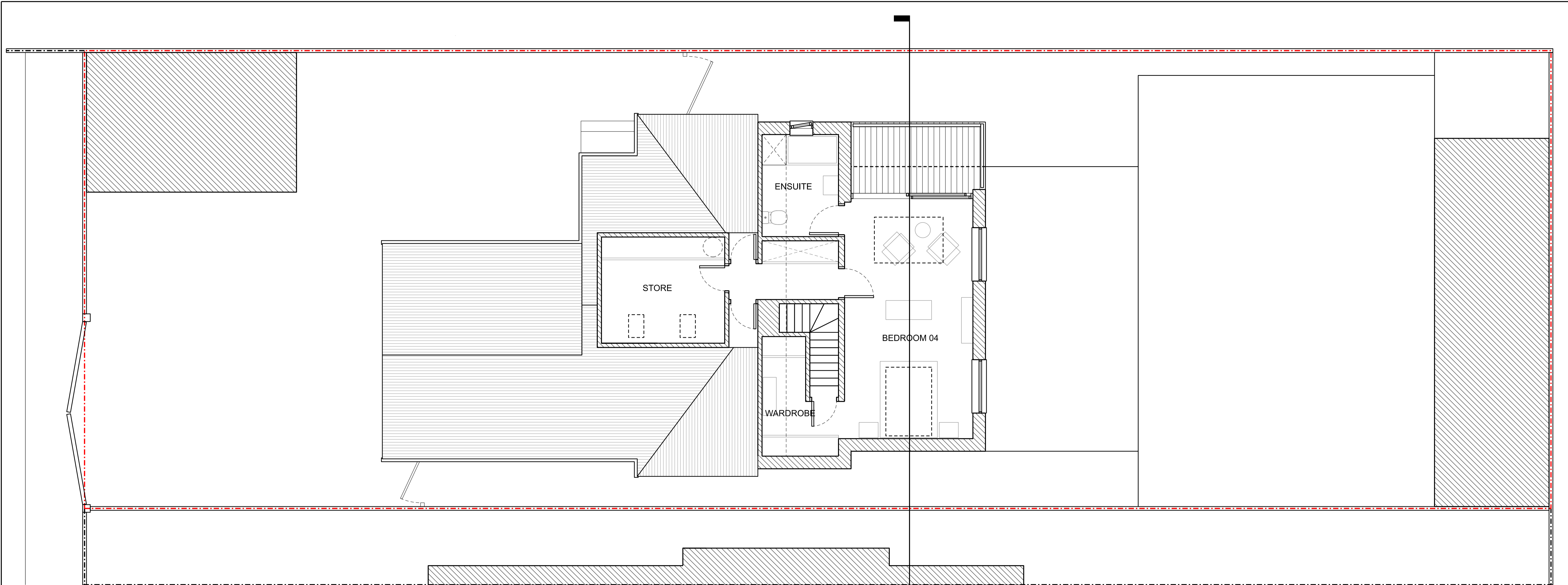
PROPOSED FIRST FLOOR PLAN 1.50@A1
