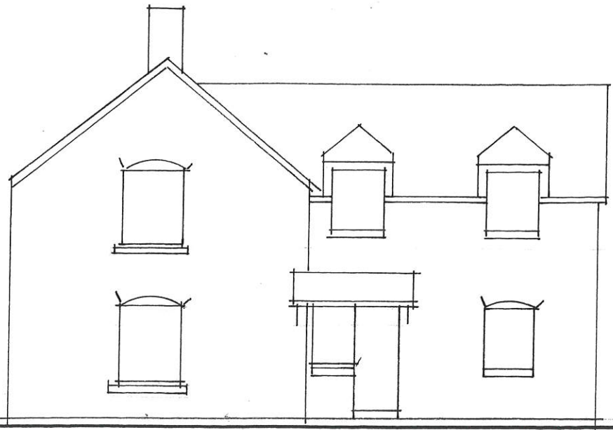
PROPOSED FRONT ELEVATION NORTH UNCHANGED 1:100
