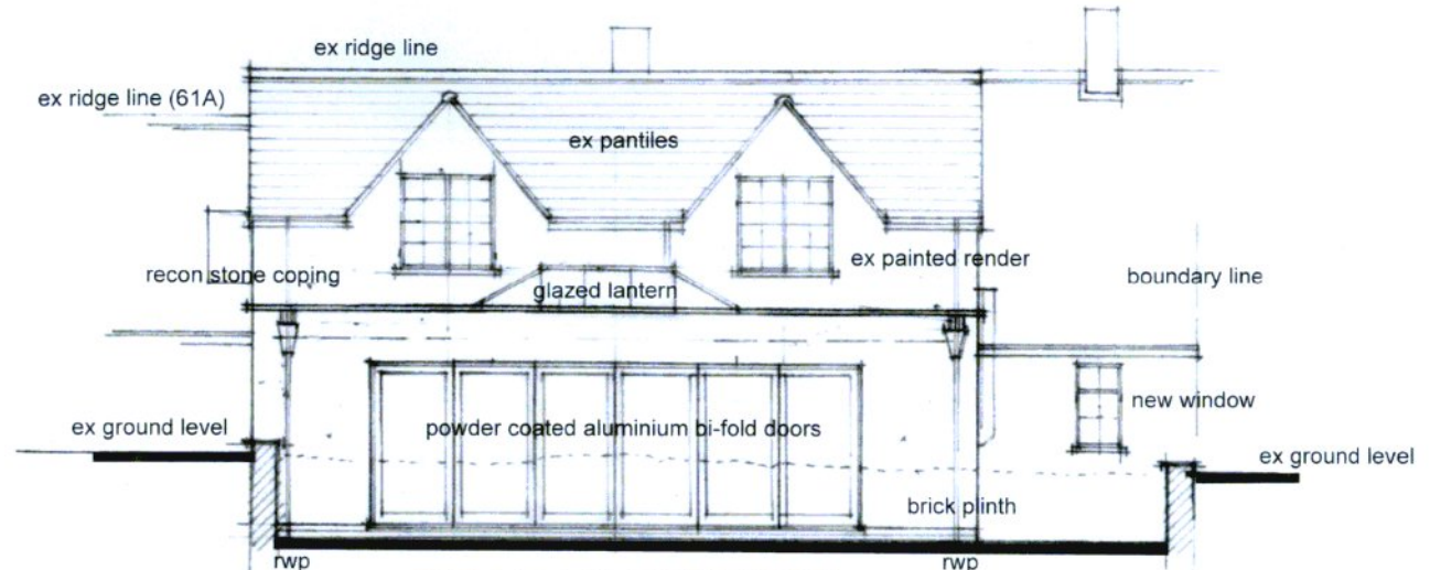
REAR ELEVATION
