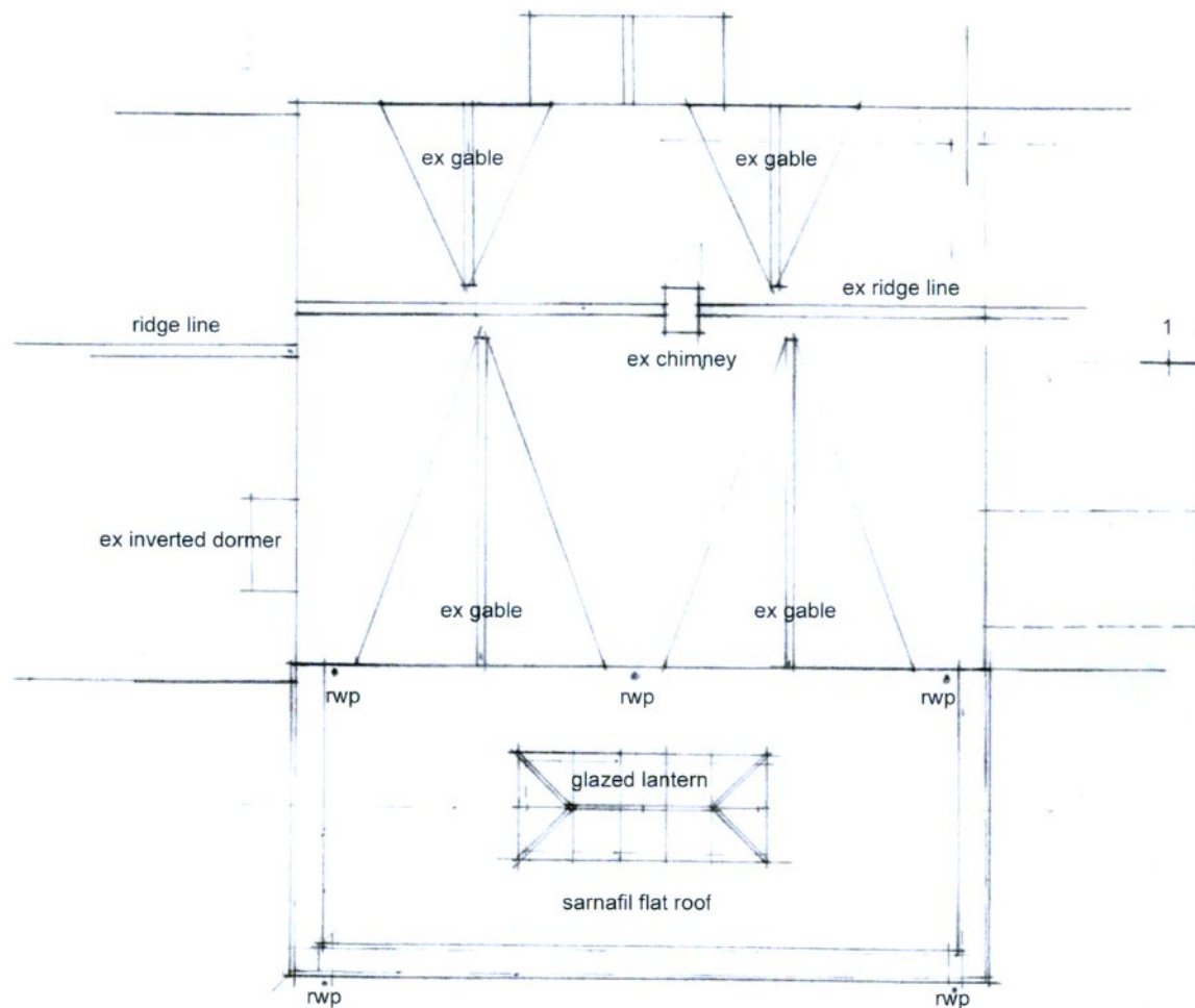
ROOF PLAN
