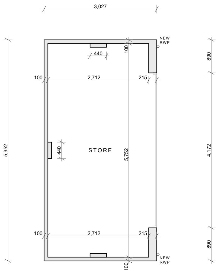
PROPOSED FLOOR PLAN LAYOUT
