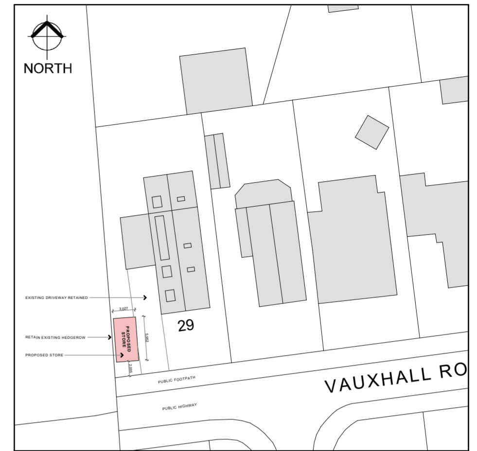
PROPOSED SITE LAYOUT PLAN (1:500)
