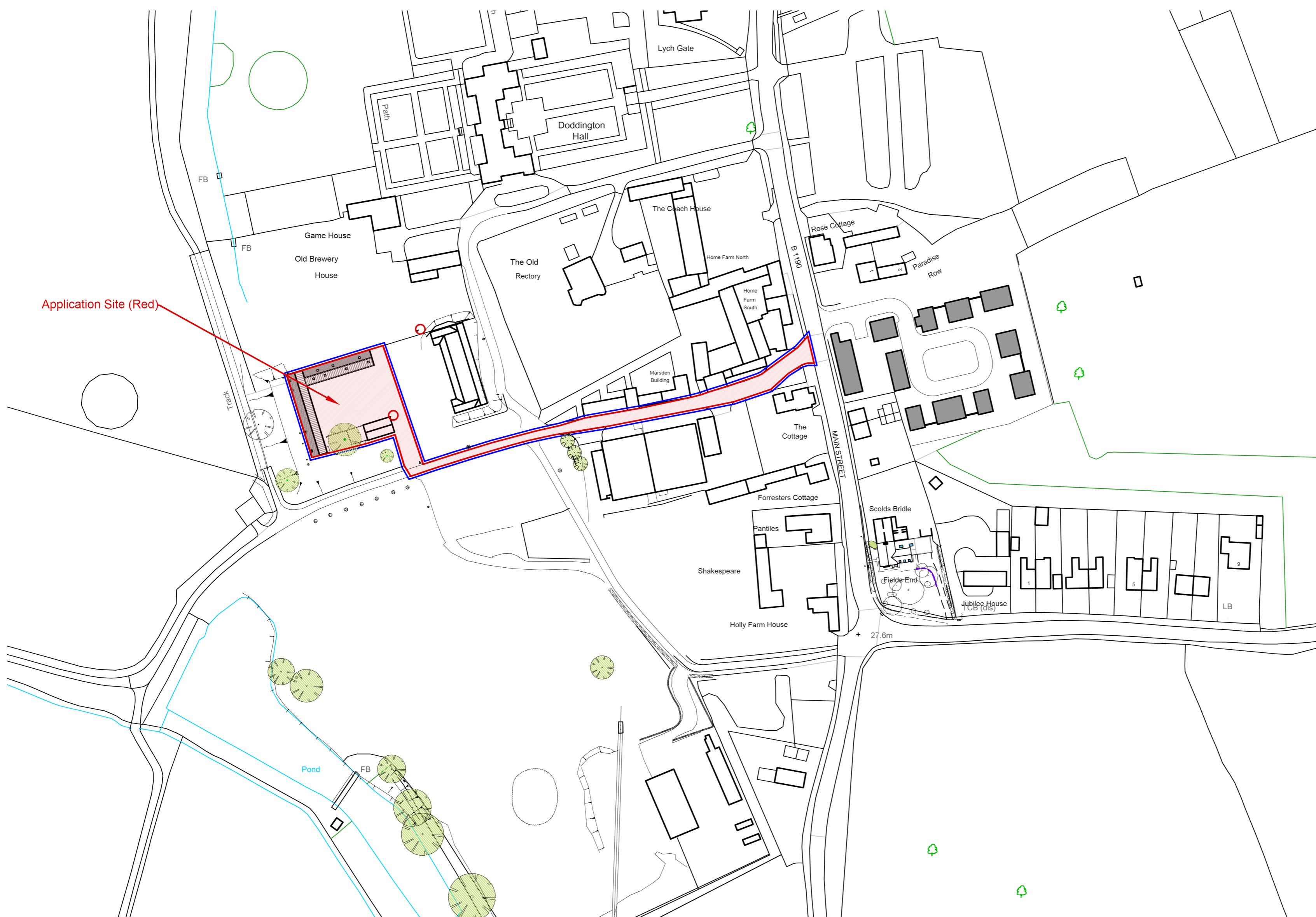
Site Location 1:1250 - A1
