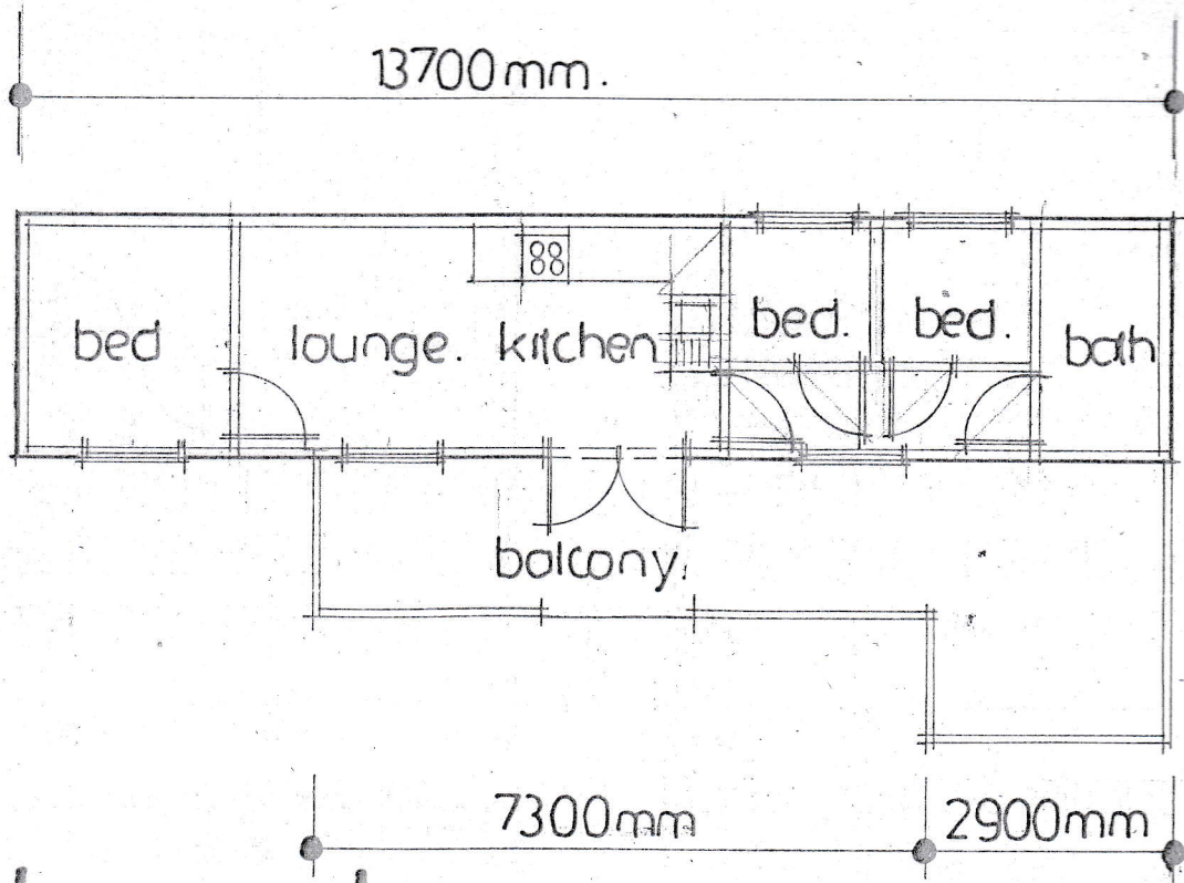
layout. 1:100.
