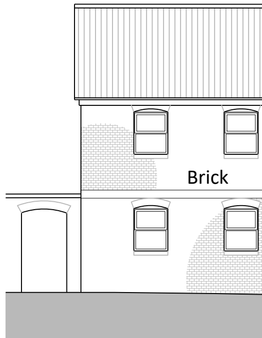
East Elevation
