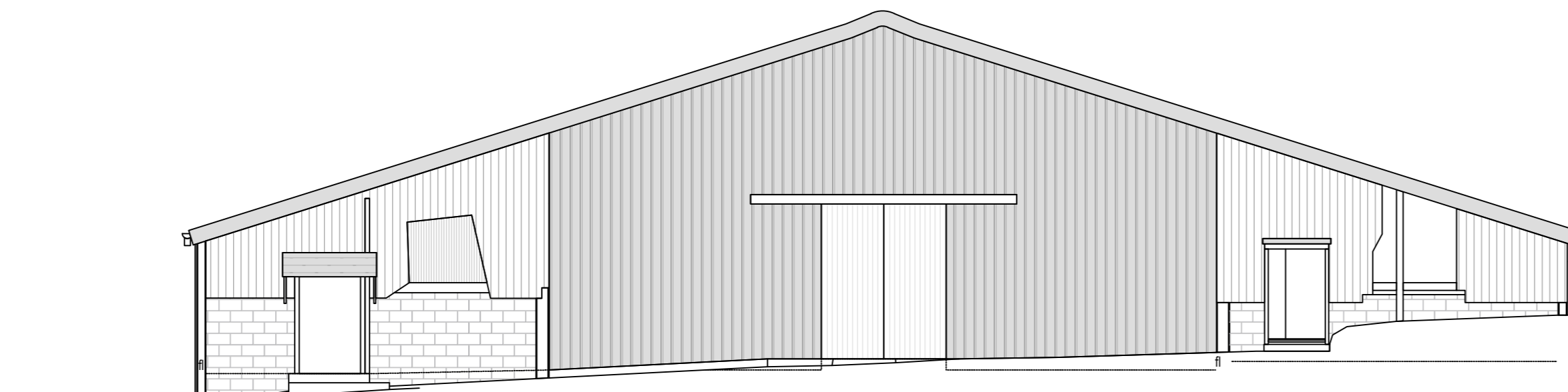
EXISTING SOUTH-EAST ELEVATION (1:100 at A0)
