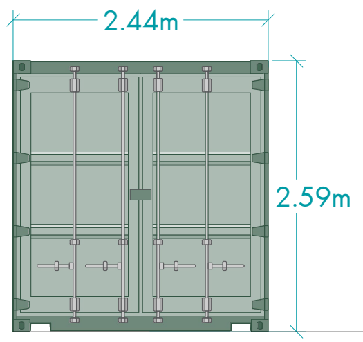
Door/End Elevation
