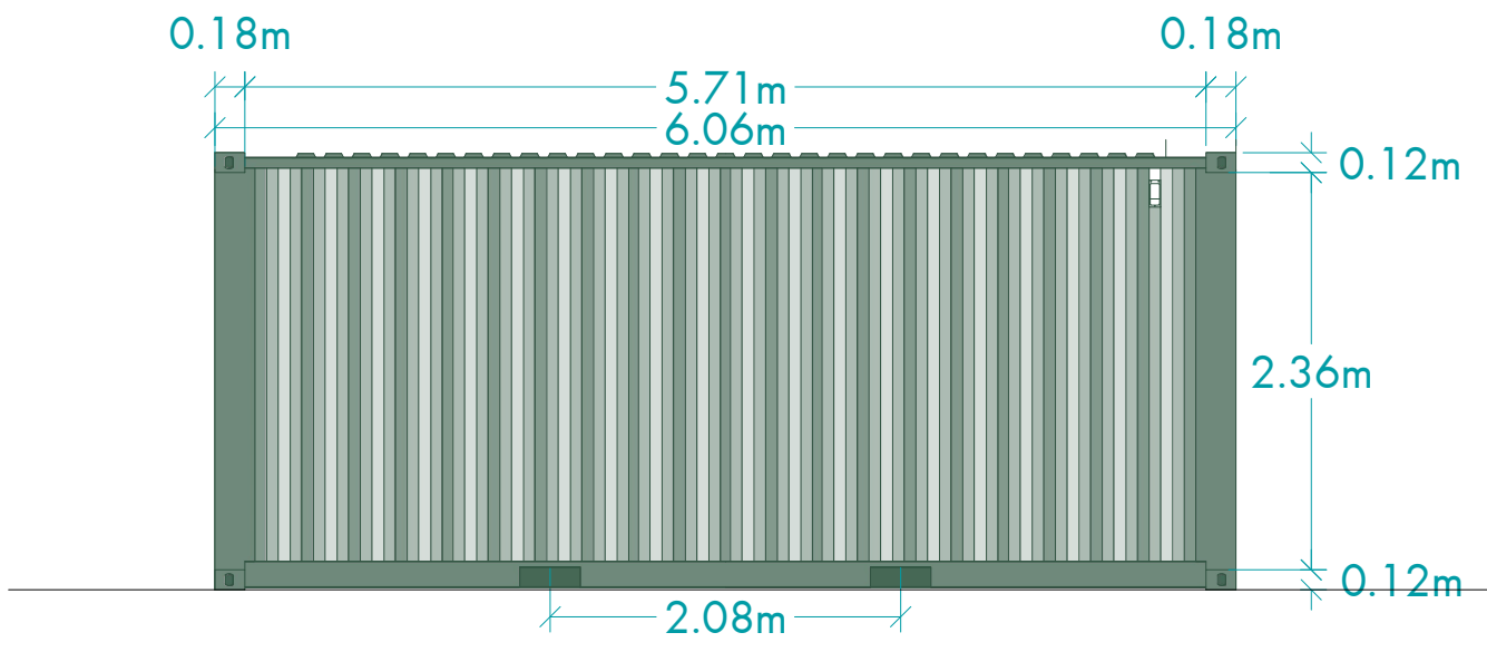
Side Elevation
