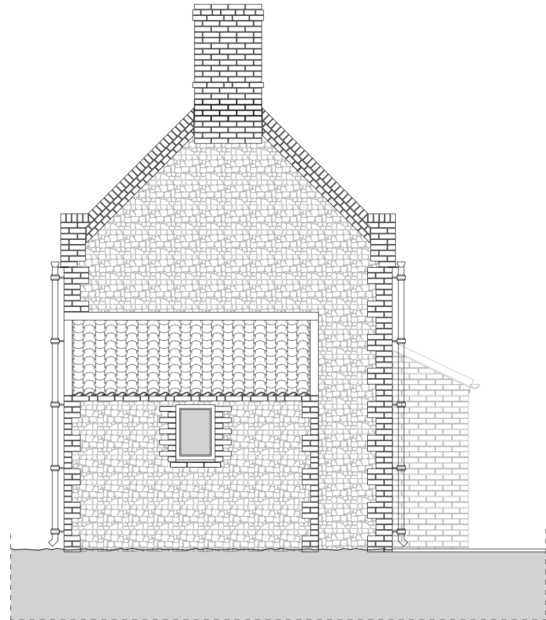
Existing West Elevation - 1:50
