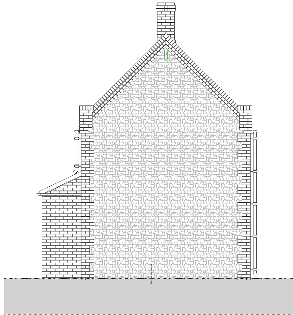
Existing East Elevation - 1:50
